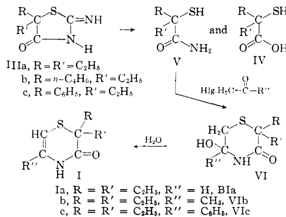
Fig. 1.—Synthesis of 2,2-trisubstituted-2,3-dihydro-4H-1,4-thiazine-3-ones.
